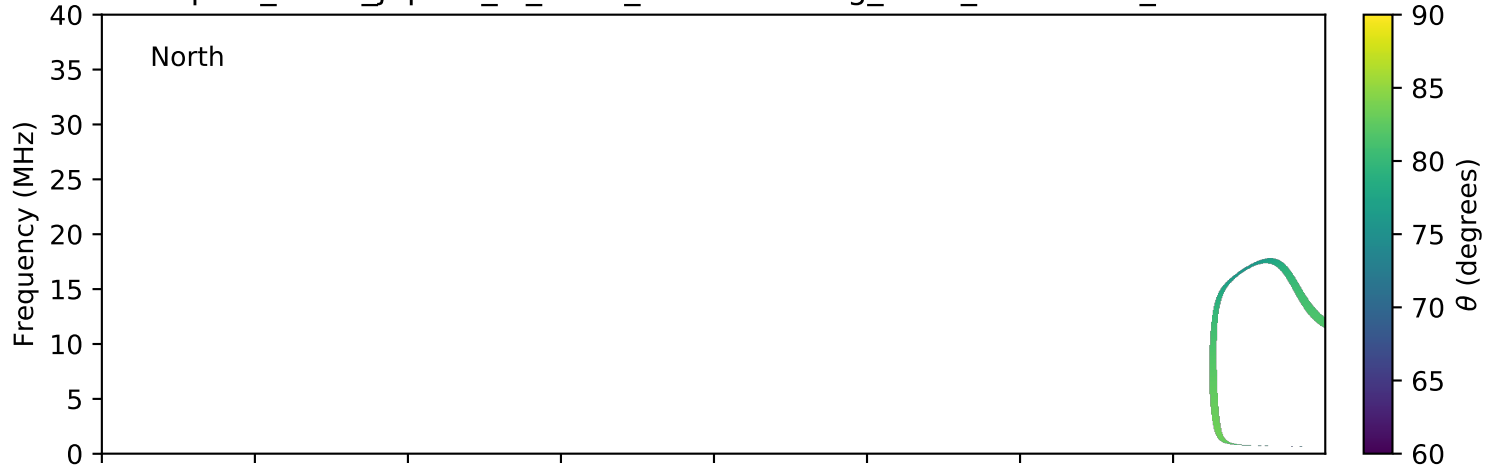
expres_earth_jupiter_io_isaac_lossc-wid1deg_3kev_20161129_v01.cdf
