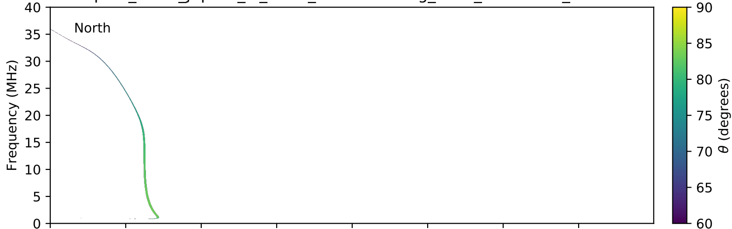
expres_earth_jupiter_io_isaac_lossc-wid1deg_3kev_20161127_v01.cdf
