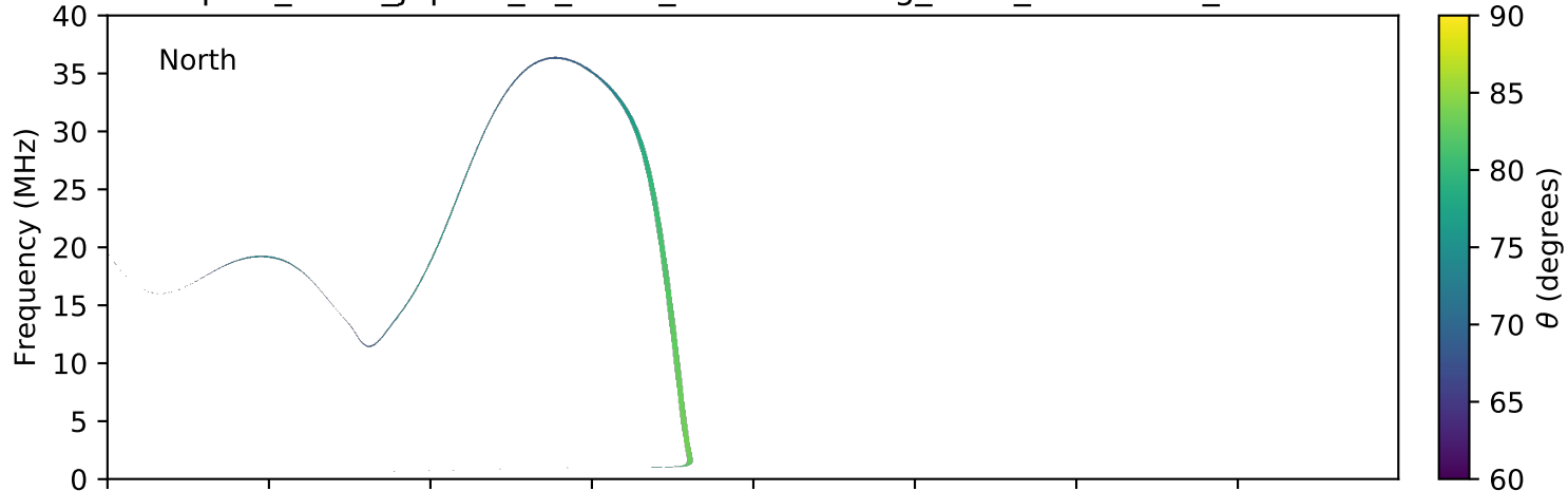
expres_earth_jupiter_io_isaac_lossc-wid1deg_3kev_20161125_v01.cdf
