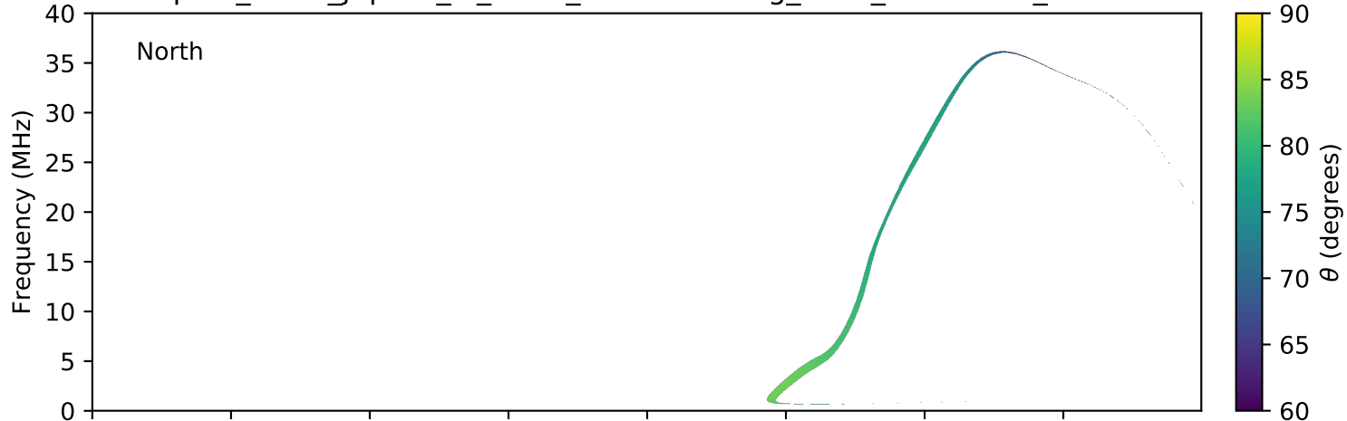
expres_earth_jupiter_io_isaac_lossc-wid1deg_3kev_20161124_v01.cdf
