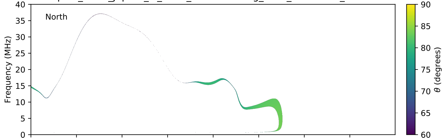
expres_earth_jupiter_io_isaac_lossc-wid1deg_3kev_20161123_v01.cdf
