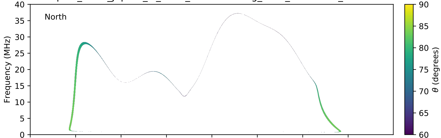
expres_earth_jupiter_io_isaac_lossc-wid1deg_3kev_20161121_v01.cdf
