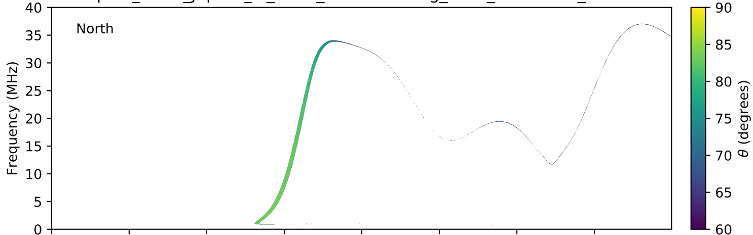
expres_earth_jupiter_io_isaac_lossc-wid1deg_3kev_20161119_v01.cdf
