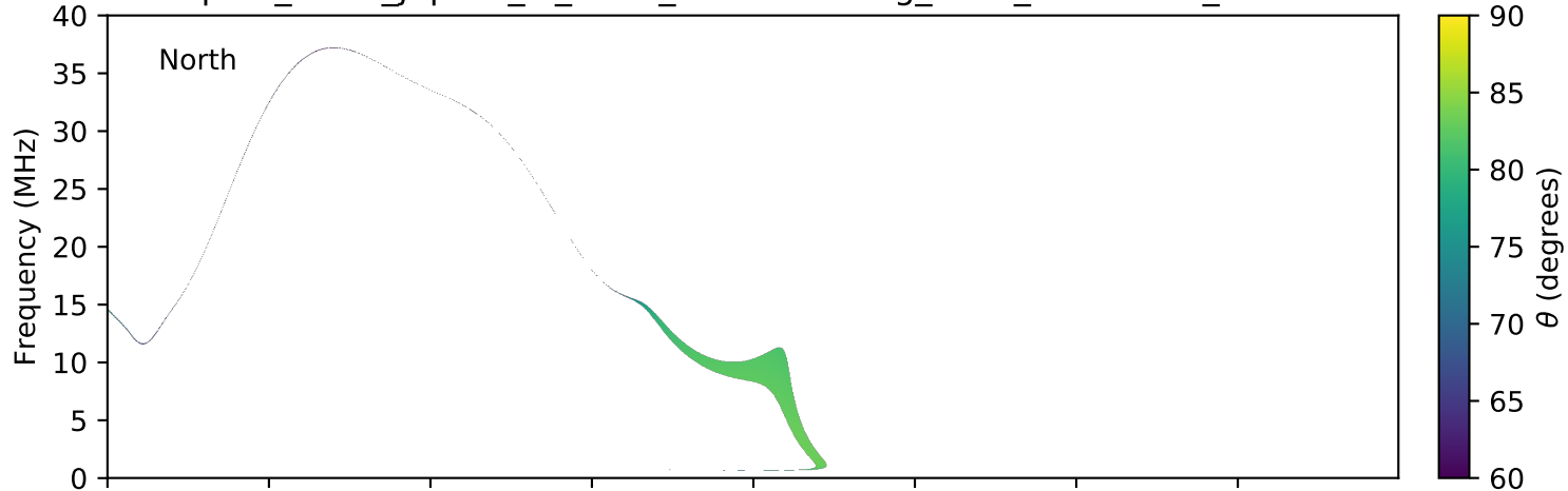
expres_earth_jupiter_io_isaac_lossc-wid1deg_3kev_20161116_v01.cdf
