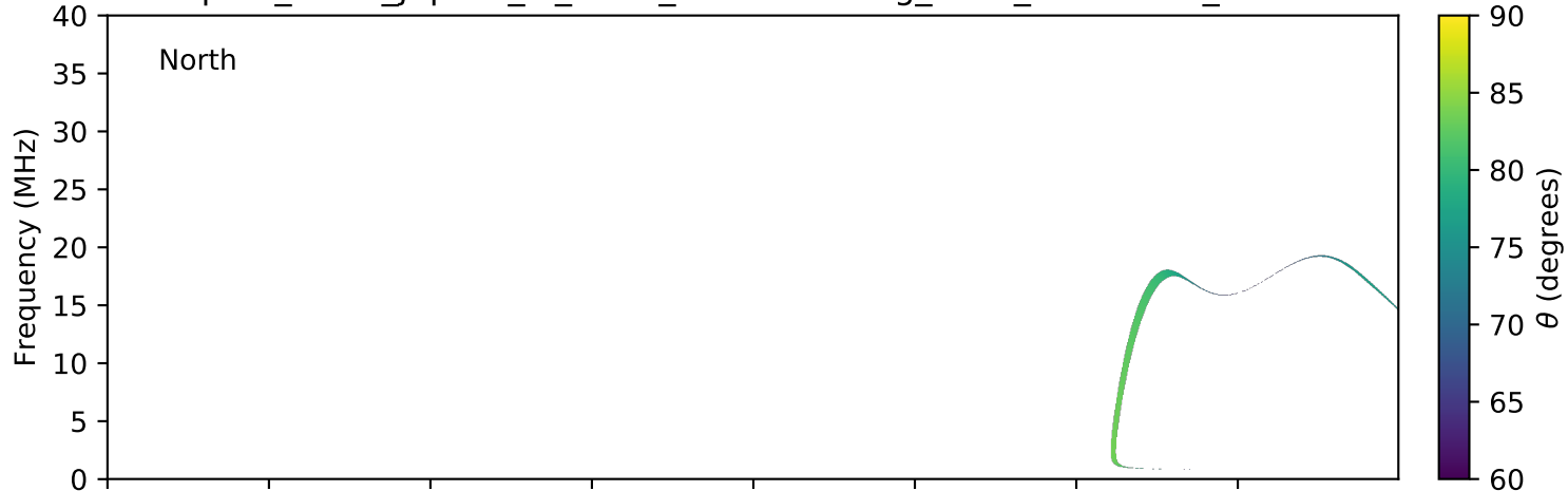
expres_earth_jupiter_io_isaac_lossc-wid1deg_3kev_20161115_v01.cdf
