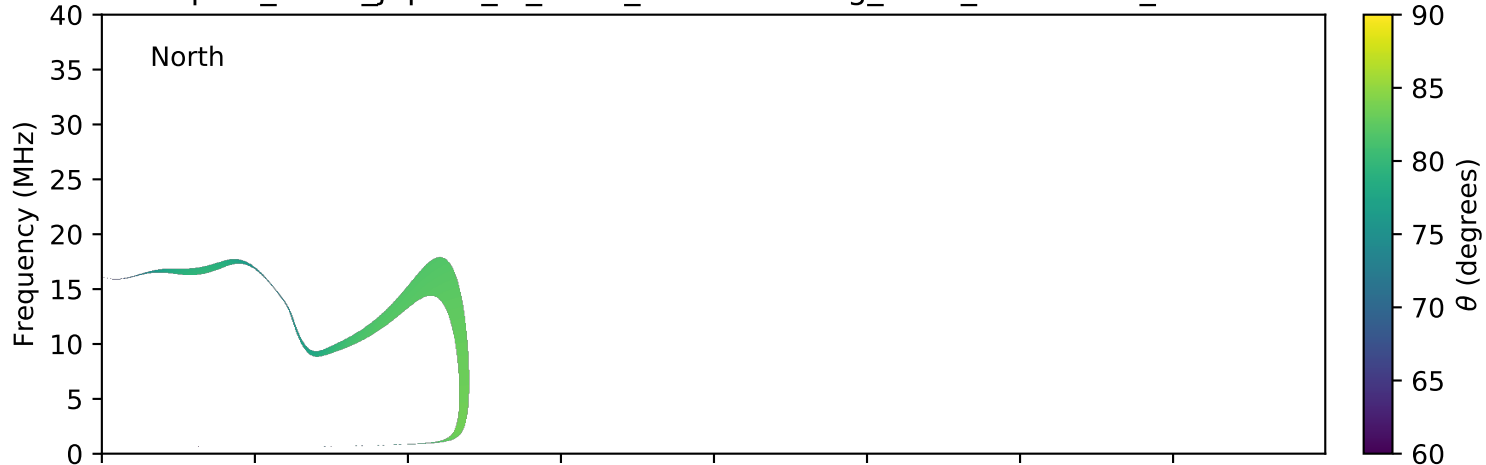
expres_earth_jupiter_io_isaac_lossc-wid1deg_3kev_20161111_v01.cdf
