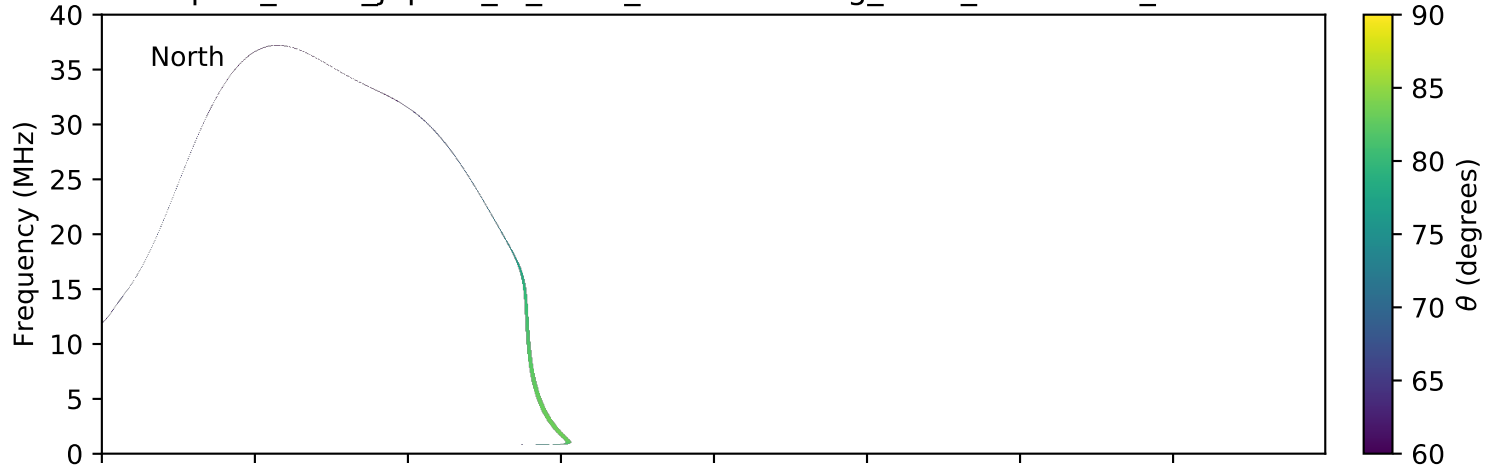
expres_earth_jupiter_io_isaac_lossc-wid1deg_3kev_20161102_v01.cdf
