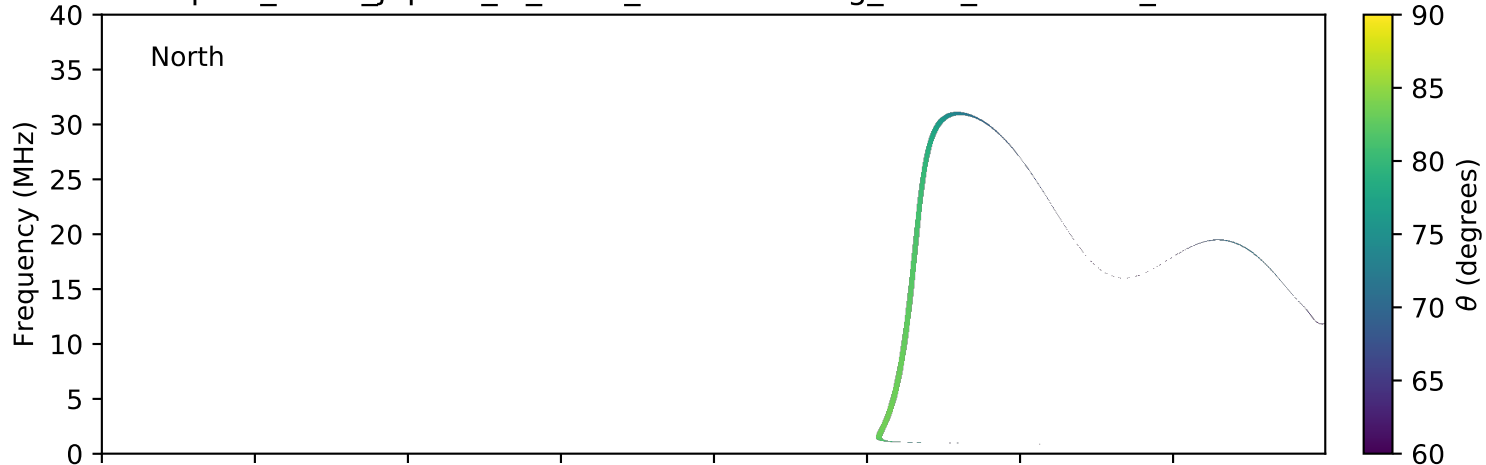
expres_earth_jupiter_io_isaac_lossc-wid1deg_3kev_20161101_v01.cdf
