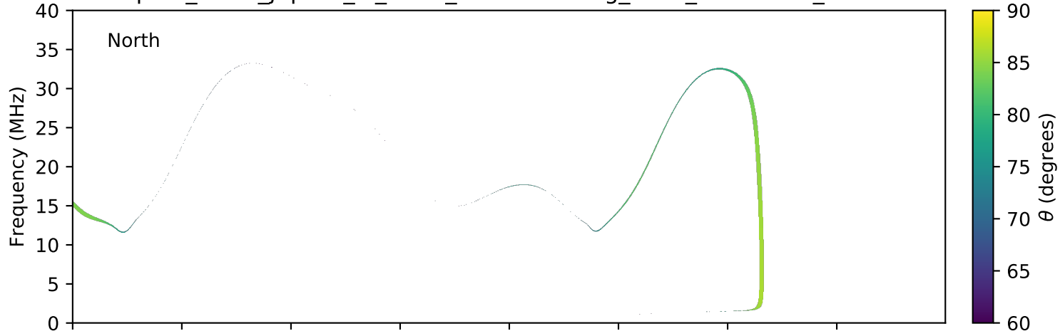
expres_earth_jupiter_io_isaac_lossc-wid1deg_1kev_20161130_v01.cdf
