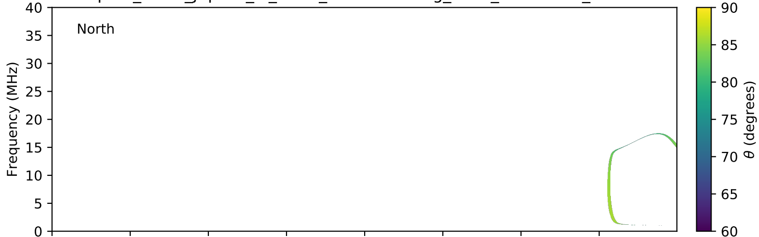
expres_earth_jupiter_io_isaac_lossc-wid1deg_1kev_20161129_v01.cdf
