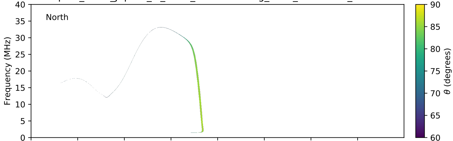
expres_earth_jupiter_io_isaac_lossc-wid1deg_1kev_20161125_v01.cdf
