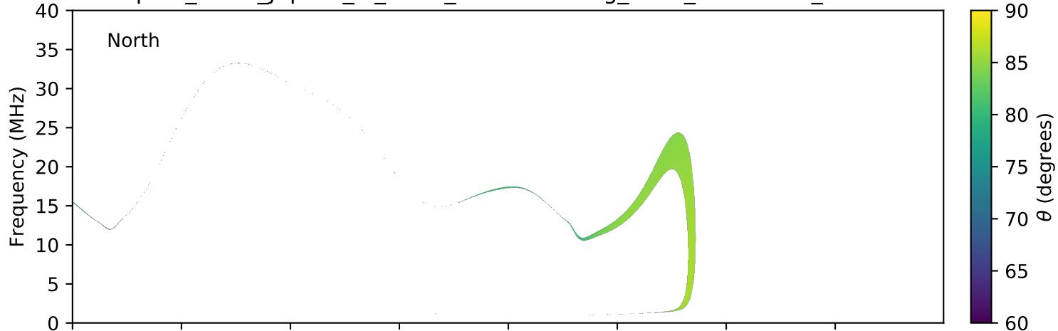
expres_earth_jupiter_io_isaac_lossc-wid1deg_1kev_20161123_v01.cdf
