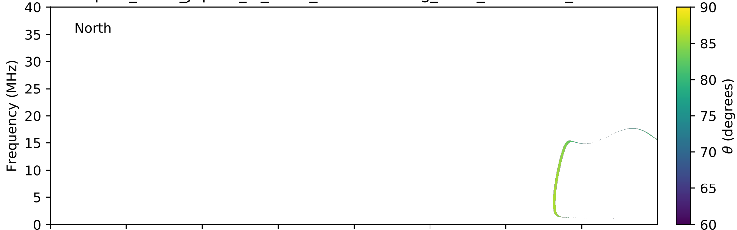
expres_earth_jupiter_io_isaac_lossc-wid1deg_1kev_20161122_v01.cdf
