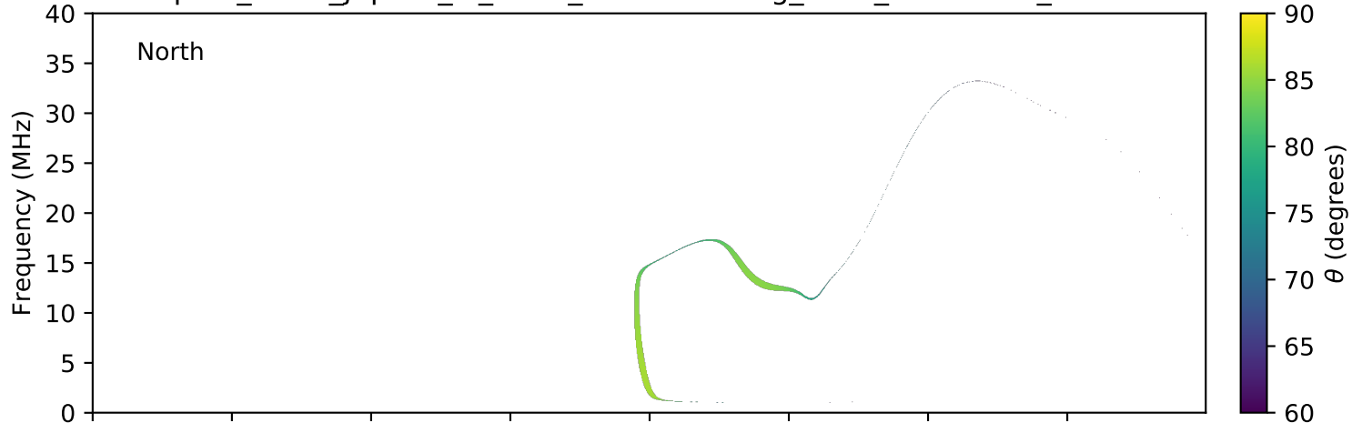
expres_earth_jupiter_io_isaac_lossc-wid1deg_1kev_20161117_v01.cdf
