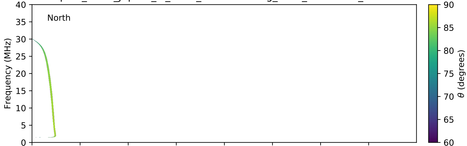
expres_earth_jupiter_io_isaac_lossc-wid1deg_1kev_20161113_v01.cdf
