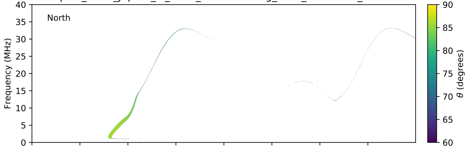
expres_earth_jupiter_io_isaac_lossc-wid1deg_1kev_20161112_v01.cdf
