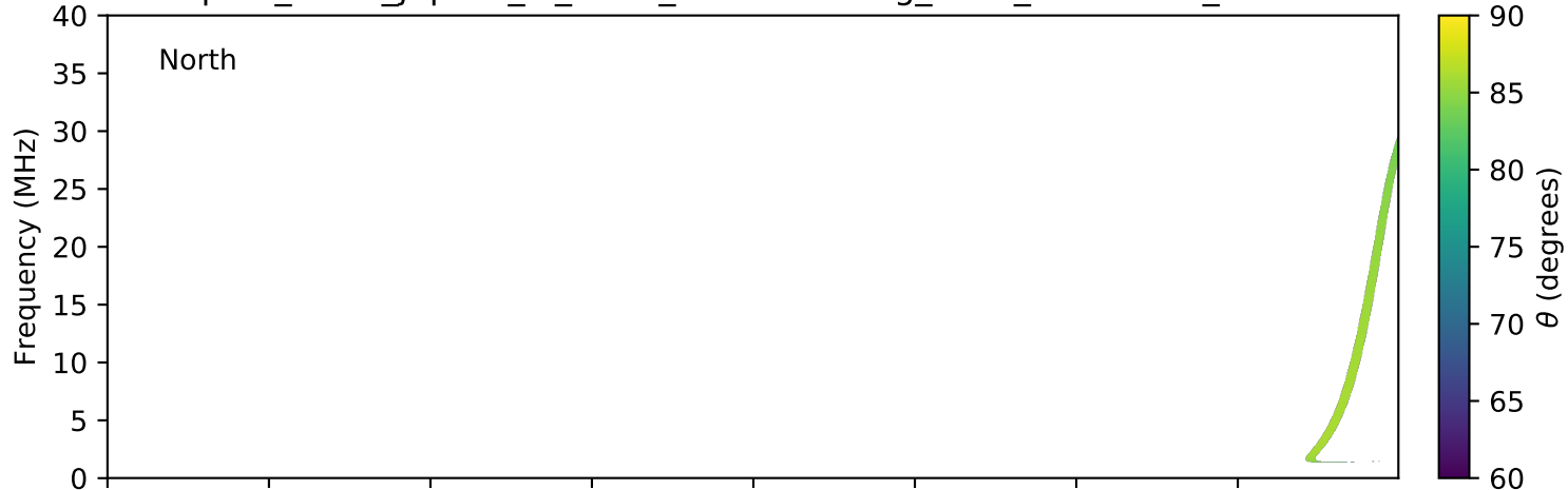
expres_earth_jupiter_io_isaac_lossc-wid1deg_1kev_20161106_v01.cdf
