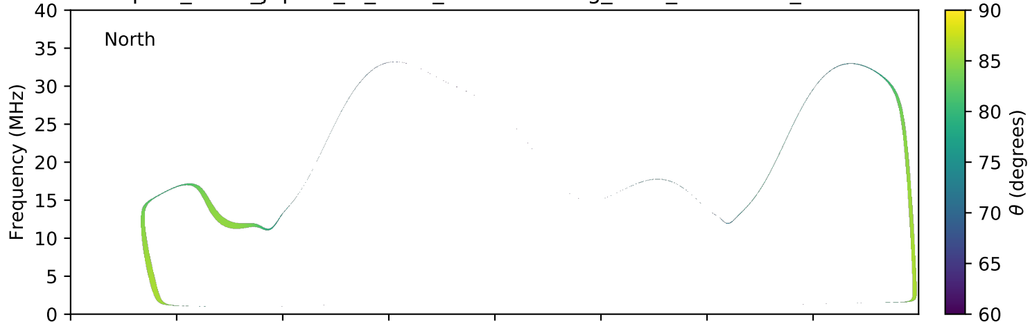
expres_earth_jupiter_io_isaac_lossc-wid1deg_1kev_20161105_v01.cdf
