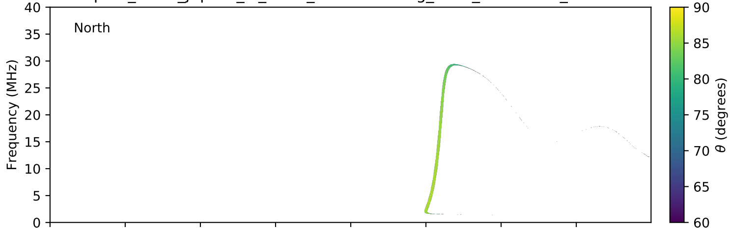
expres_earth_jupiter_io_isaac_lossc-wid1deg_1kev_20161101_v01.cdf
