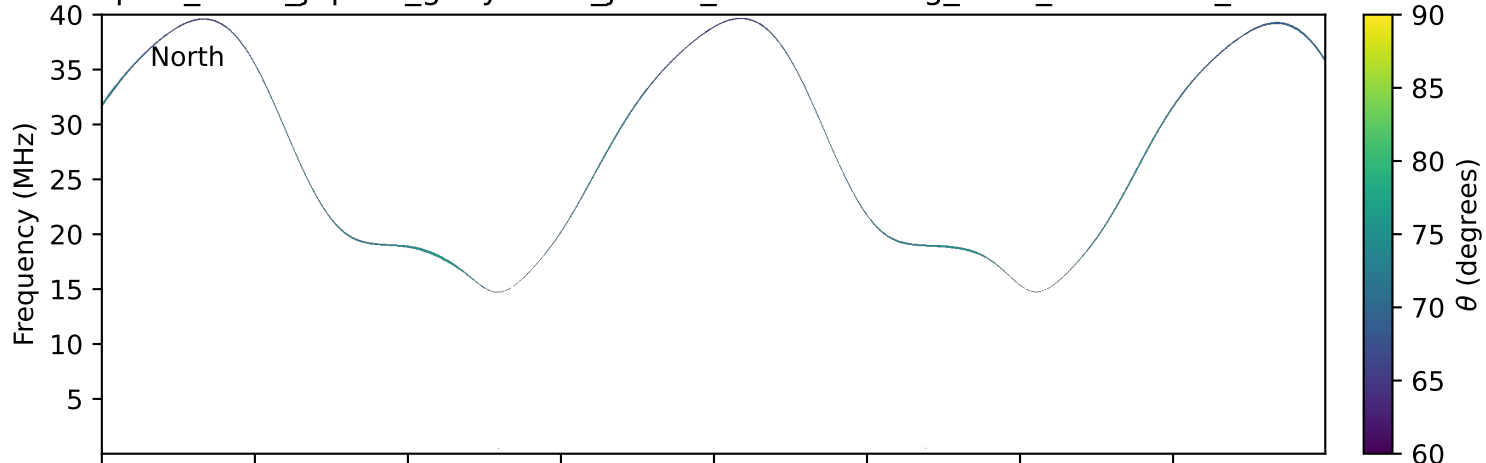
expres_earth_jupiter_ganymede_jrm33_lossc-wid1deg_3kev_20161112_v11.cdf
