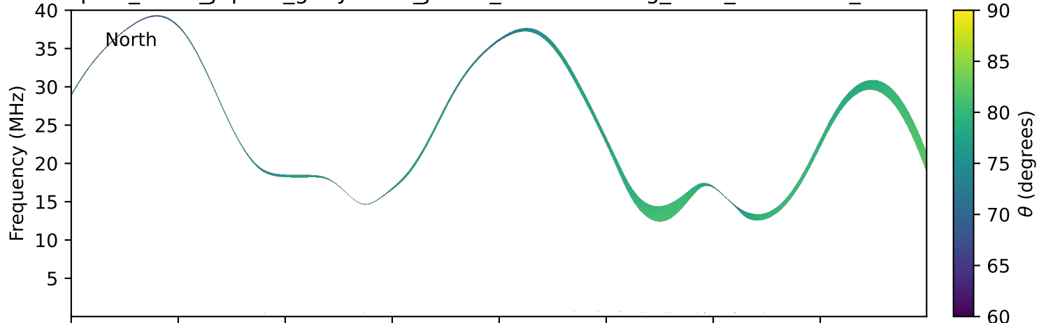
expres_earth_jupiter_ganymede_jrm33_lossc-wid1deg_3kev_20161105_v11.cdf
