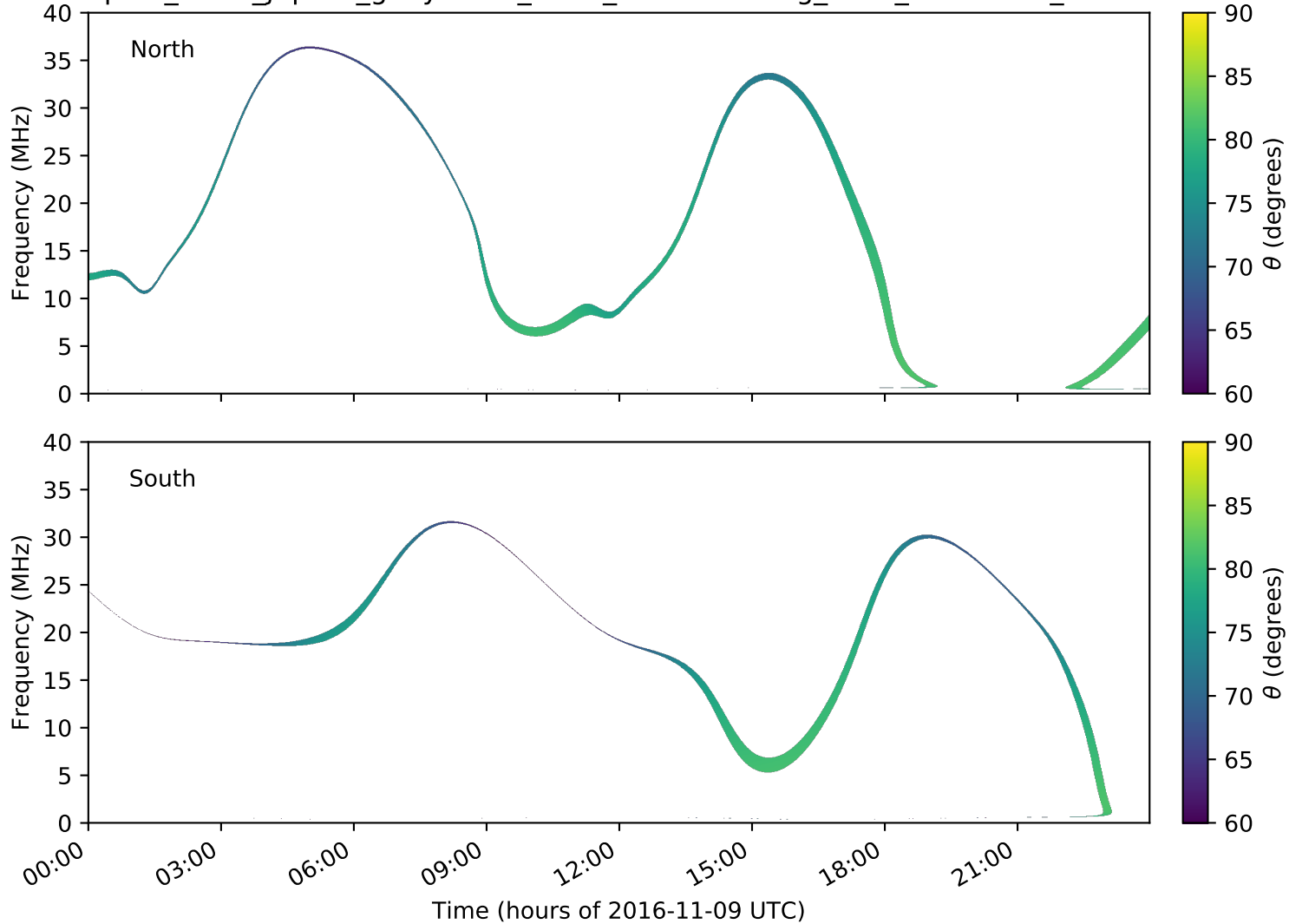
expres_earth_jupiter_ganymede_isaac_lossc-wid1deg_5kev_20161109_v01.cdf
