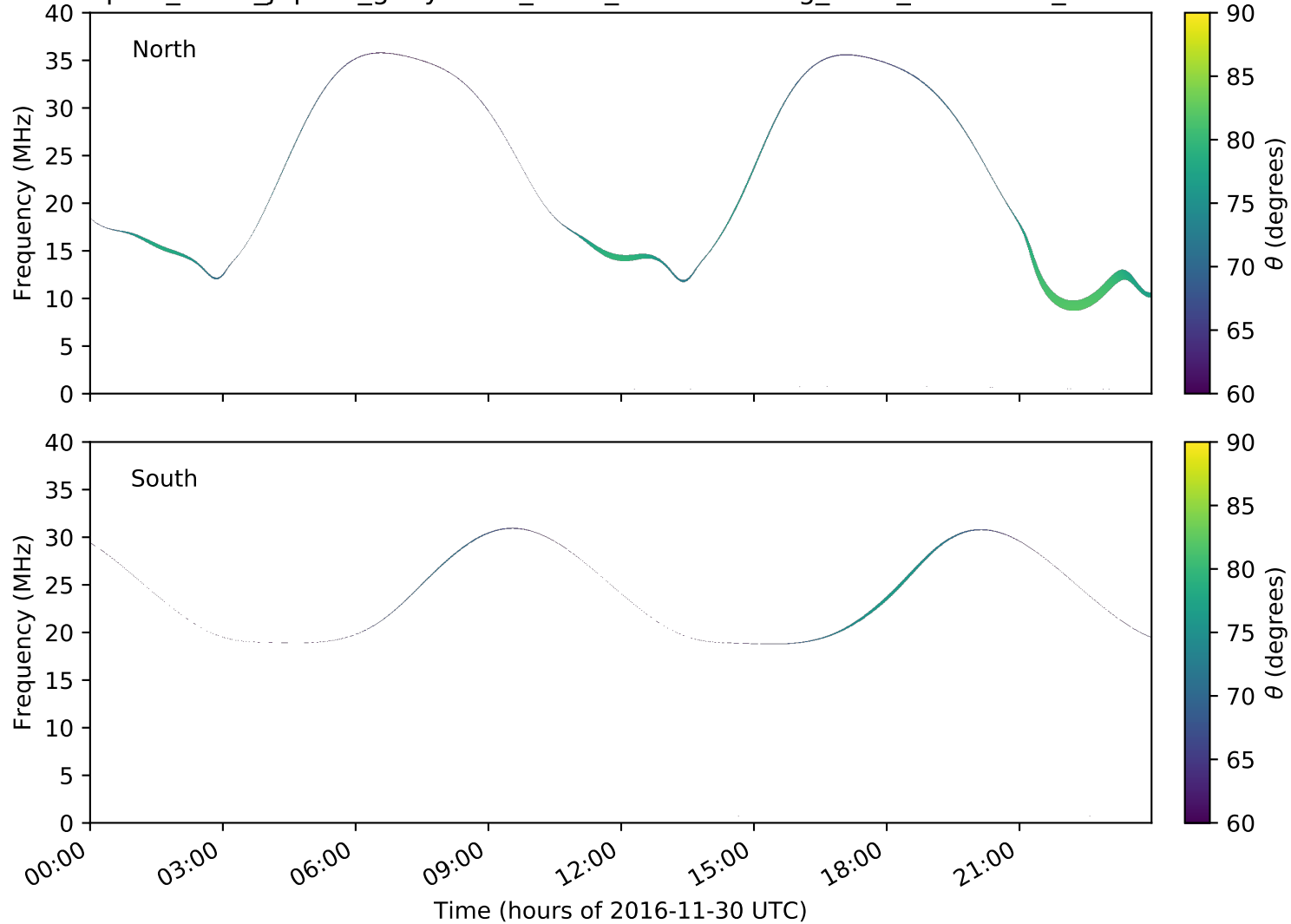
expres_earth_jupiter_ganymede_isaac_lossc-wid1deg_3kev_20161130_v01.cdf
