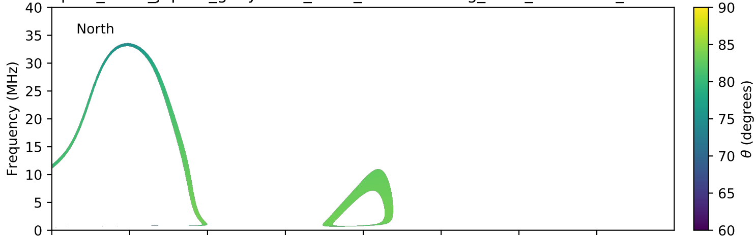
expres_earth_jupiter_ganymede_isaac_lossc-wid1deg_3kev_20161124_v01.cdf
