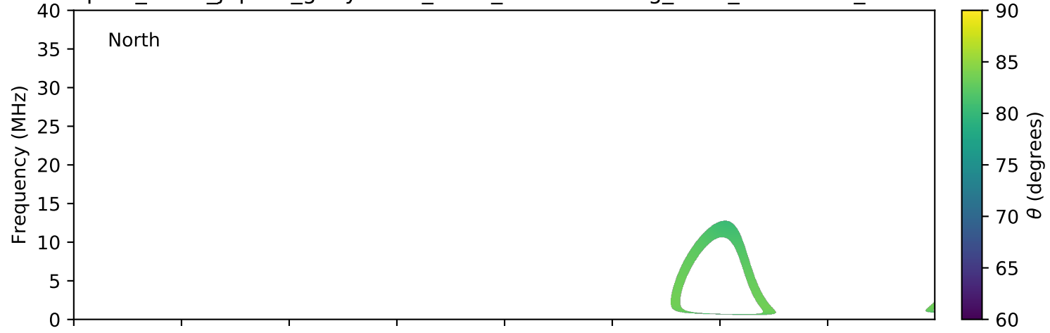
expres_earth_jupiter_ganymede_isaac_lossc-wid1deg_3kev_20161106_v01.cdf
