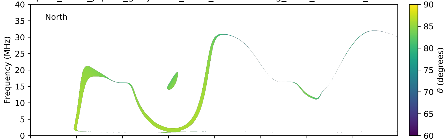
expres_earth_jupiter_ganymede_isaac_lossc-wid1deg_1kev_20161121_v01.cdf
