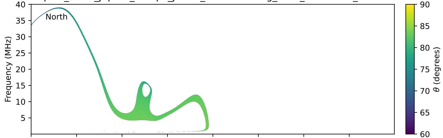
expres_earth_jupiter_europa_jrm33_lossc-wid1deg_3kev_20161122_v11.cdf
