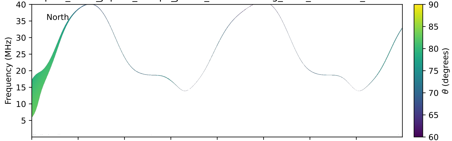
expres_earth_jupiter_europa_jrm33_lossc-wid1deg_3kev_20161121_v11.cdf
