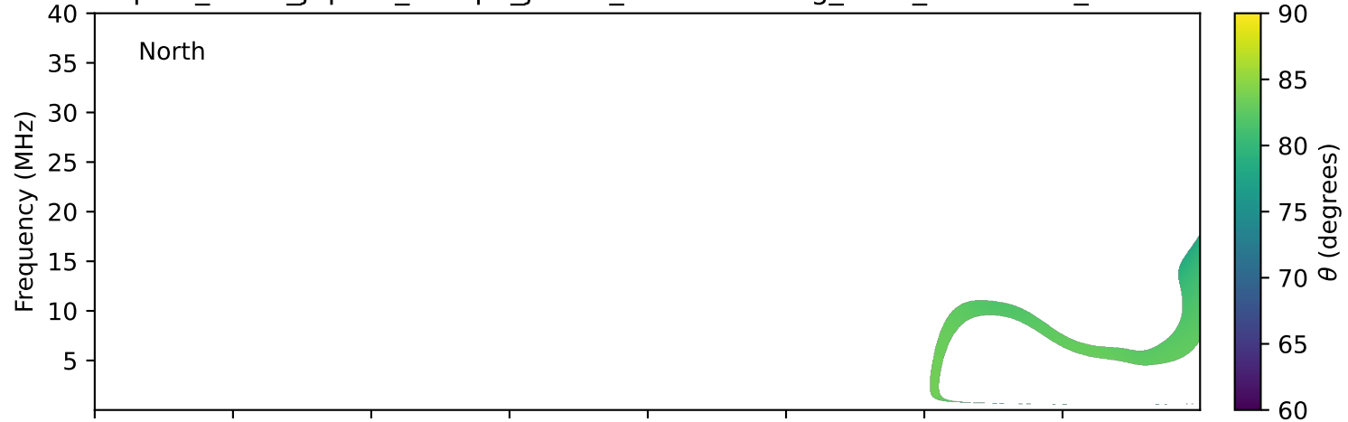
expres_earth_jupiter_europa_jrm33_lossc-wid1deg_3kev_20161120_v11.cdf
