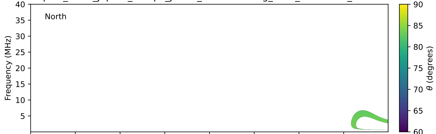
expres_earth_jupiter_europa_jrm33_lossc-wid1deg_3kev_20161105_v11.cdf
