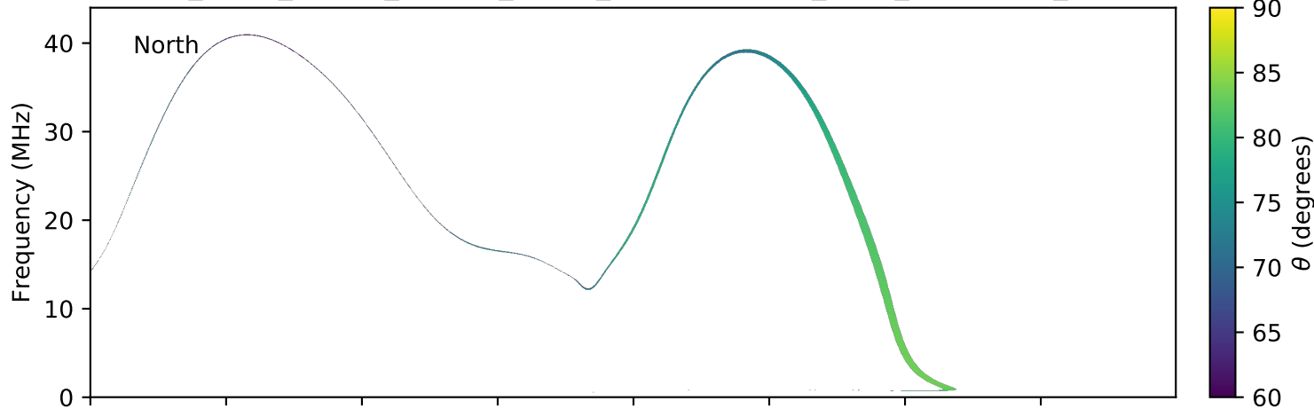
expres_earth_jupiter_europa_jrm09_lossc-wid1deg_3kev_20161126_v01.cdf
