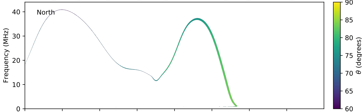
expres_earth_jupiter_europa_jrm09_lossc-wid1deg_3kev_20161119_v01.cdf
