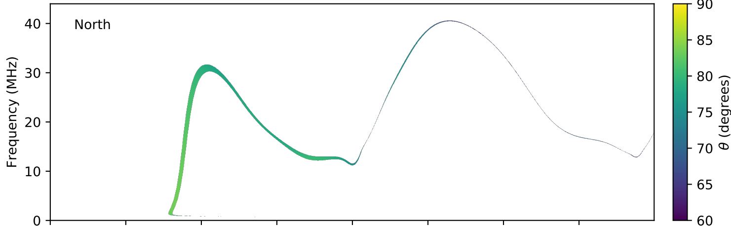
expres_earth_jupiter_europa_jrm09_lossc-wid1deg_3kev_20161118_v01.cdf
