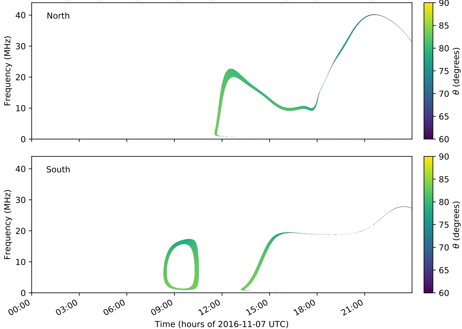
expres_earth_jupiter_europa_jrm09_lossc-wid1deg_3kev_20161107_v01.cdf
