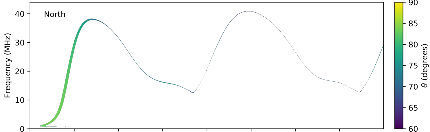
expres_earth_jupiter_europa_jrm09_lossc-wid1deg_3kev_20161104_v01.cdf
