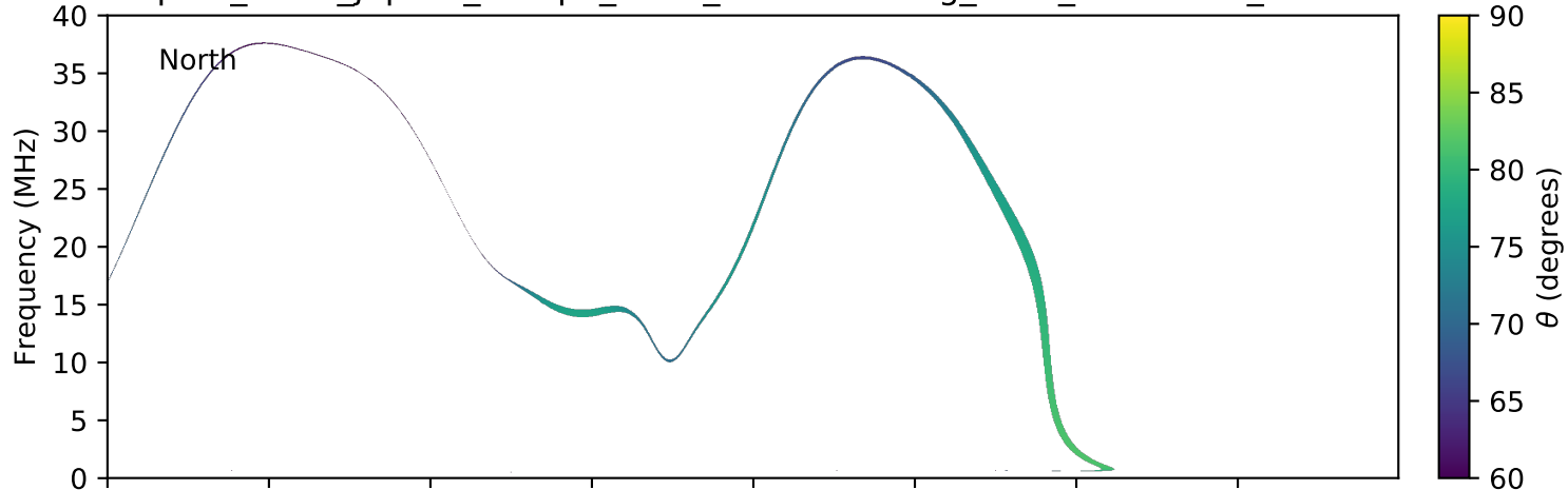
expres_earth_jupiter_europa_isaac_lossc-wid1deg_5kev_20161126_v01.cdf
