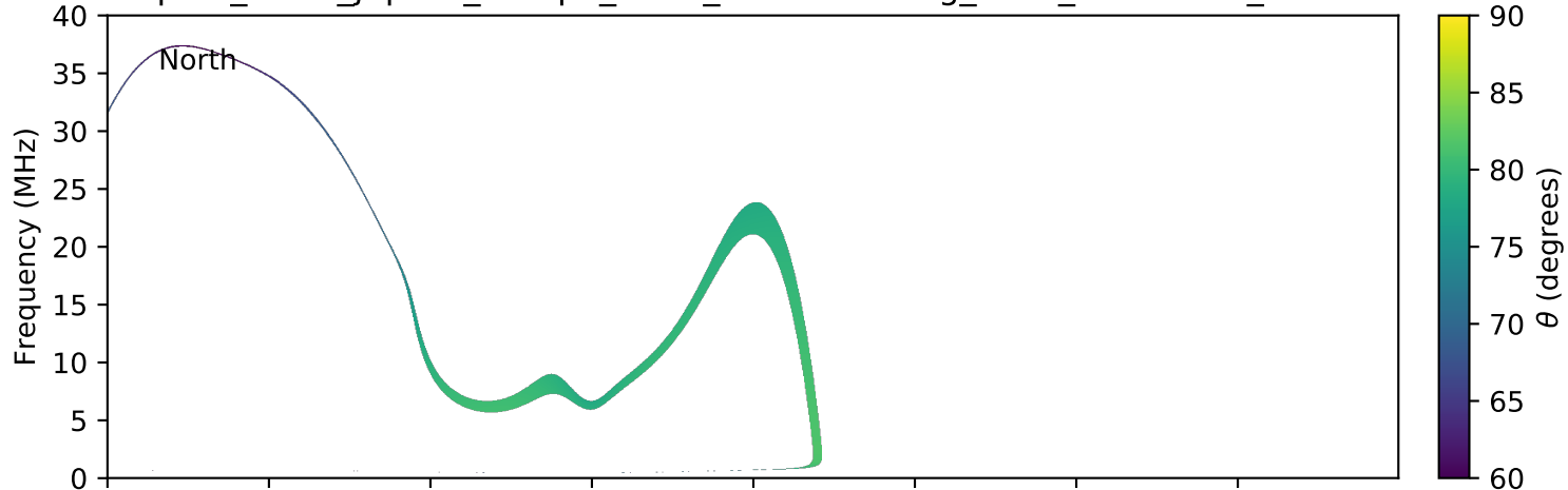
expres_earth_jupiter_europa_isaac_lossc-wid1deg_5kev_20161105_v01.cdf
