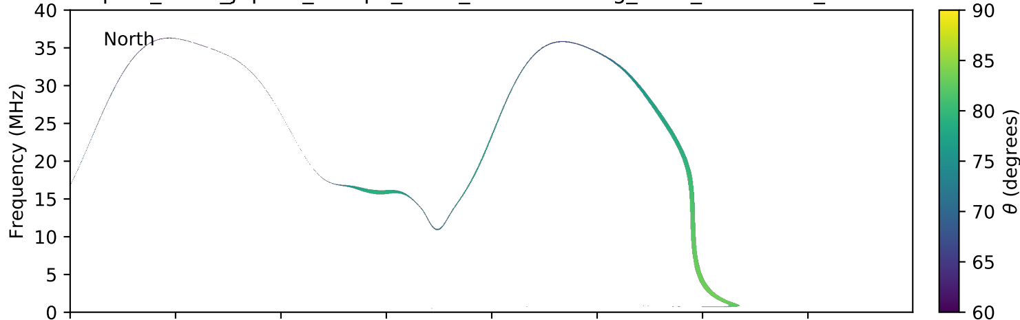
expres_earth_jupiter_europa_isaac_lossc-wid1deg_3kev_20161126_v01.cdf
