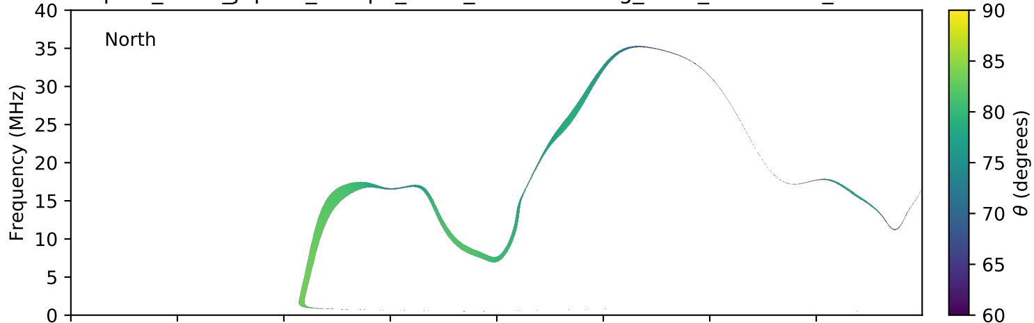
expres_earth_jupiter_europa_isaac_lossc-wid1deg_3kev_20161125_v01.cdf
