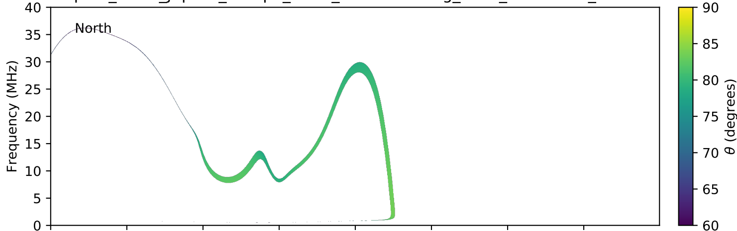
expres_earth_jupiter_europa_isaac_lossc-wid1deg_3kev_20161105_v01.cdf
