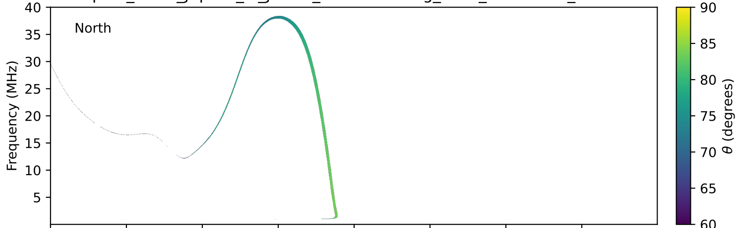
expres_earth_jupiter_io_jrm33_lossc-wid1deg_3kev_20161020_v11.cdf
