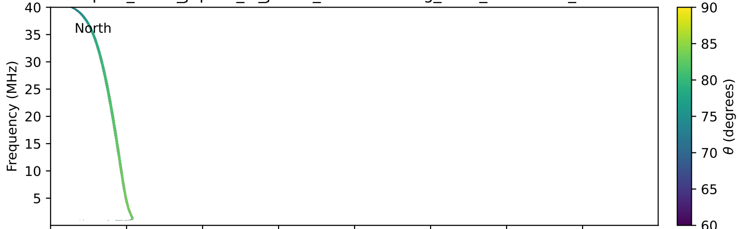
expres_earth_jupiter_io_jrm33_lossc-wid1deg_3kev_20161015_v11.cdf
