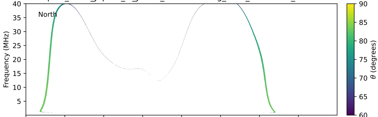
expres_earth_jupiter_io_jrm33_lossc-wid1deg_3kev_20161009_v11.cdf
