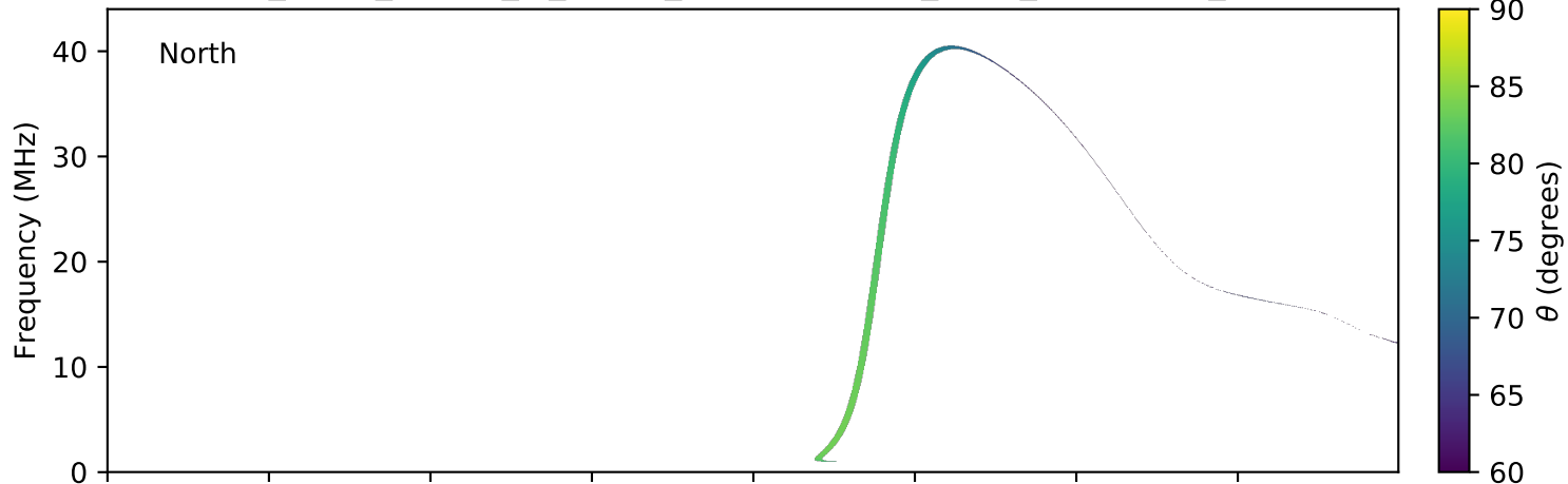
expres_earth_jupiter_io_jrm09_lossc-wid1deg_3kev_20161025_v01.cdf
