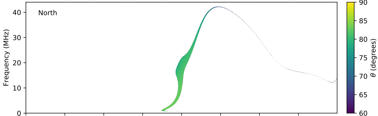
expres_earth_jupiter_io_jrm09_lossc-wid1deg_3kev_20161018_v01.cdf
