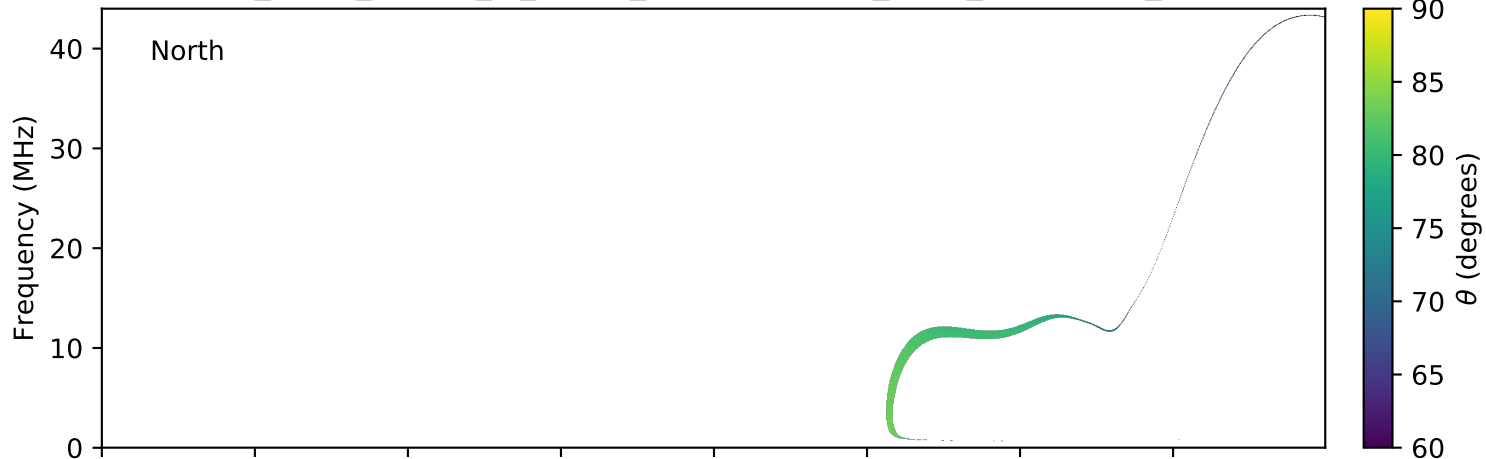
expres_earth_jupiter_io_jrm09_lossc-wid1deg_3kev_20161016_v01.cdf
